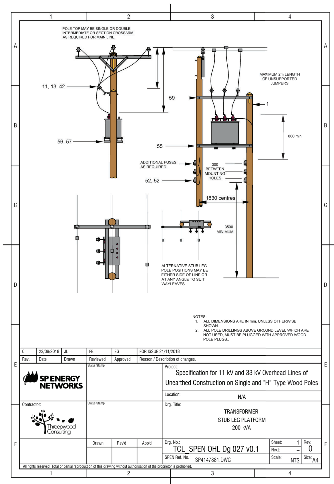
22.27 Figure 27 General Arrangement Transformer Stub Leg Platform 200kVA (Drawing No. SP4147881)
